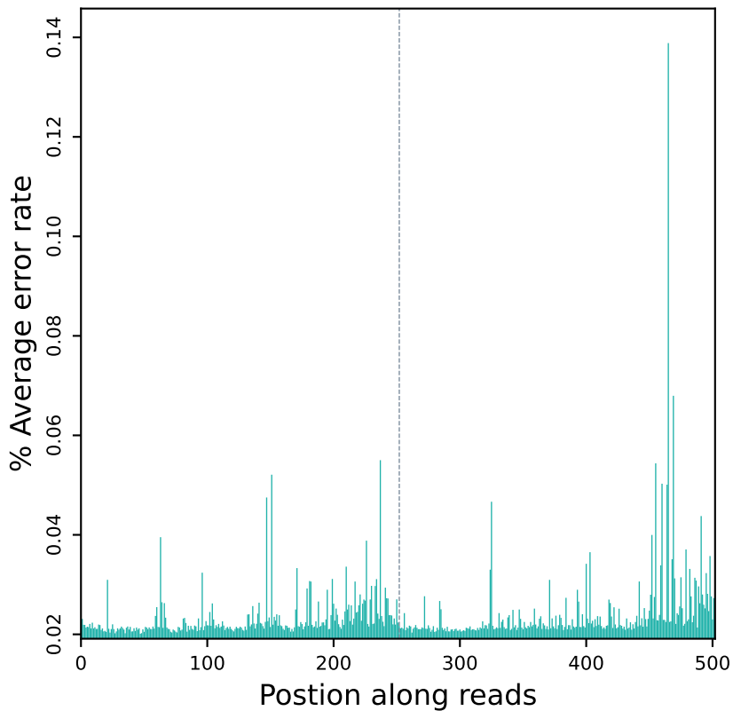
Error rate distribution along reads (R10925)
